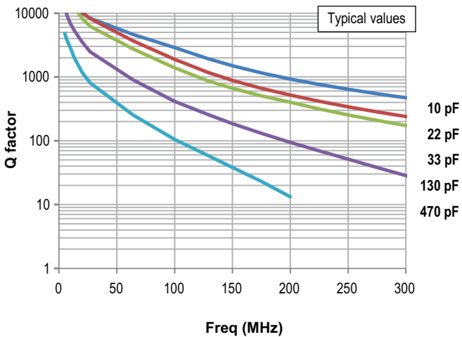
2525 - Q factor
