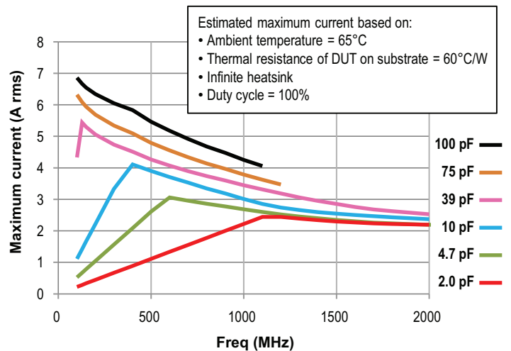
0603 - Max Current
